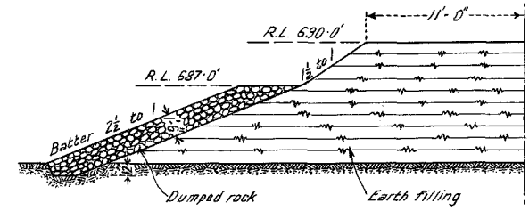
- SECTION Z-Z -
