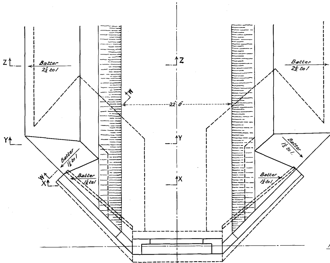
- PLAN -
