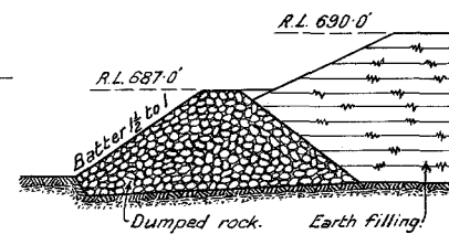
- SECTION W-W -
